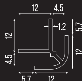
Buitenhoek 4mm
