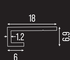
Endcap 4mm
