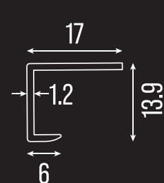
Endcap 11mm
