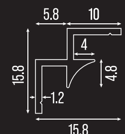
Binnenhoek 4mm
